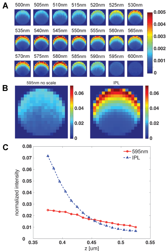
Fig. 4. (A) Normalized absorbed energy distribution within 0.081 \mu\text{m} radius vessel over 500–600 nm wavelength range at 5 nm increments. All energy distribution maps are plotted on the same color scale. (B) Comparison of 595 nm normalized absorbed energy distribution and composite narrowband IPL 500–60 nm energy distribution of 0.081 \mu\text{m} radius vessel. The average absorbed energy in the upper half of the line profile of the IPL is 0.0406 \pm 0.0004 while the average in the lower half is 0.0098 \pm 0.0003. At 595 nm the average absorbed energy in the upper half is 0.0216 \pm 0.0004 and in the lower half is 0.0131 \pm 0.0003. Composite vessel indicates that most absorbed energy is contained within the top half of the vessel, while the bottom half has lower absorbed energy compared to 595 nm. (C) Line profile of normalized absorbed energy distribution with one-sigma error bars (bars are smaller than symbol) using 595 nm and narrowband IPL irradiation. With the former, the average absorbed energy is more evenly distributed over the entire vessel, as compared to the narrowband IPL absorbed energy.
